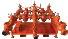
Circulating Manifolds
